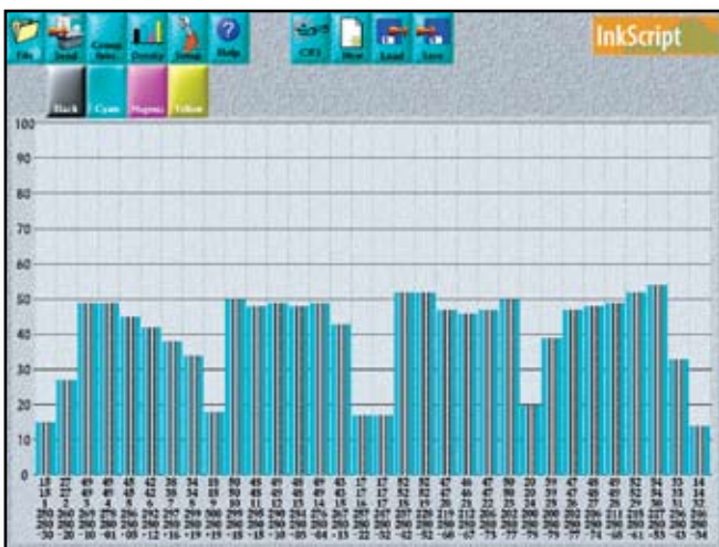
Output: Transmitting correction values to the printing press
